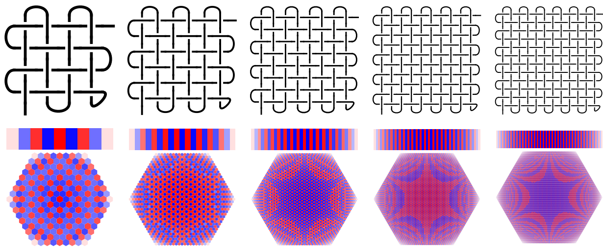
FIGURE 1.2. \Theta of some square weave knots, as computed by Self [BV3, WeaveKnots.nb].
