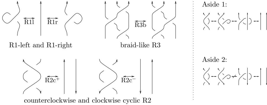
FIGURE 4.2. A generating set of oriented Reidemeister moves as in [Po2, Figure 6]. Aside 1: the braid-like R2b is not needed. Aside 2: yet R2b cannot replace R2c^\pm because in the would-be proof, an unpostulated form of R3 is used (which in itself follows from R2c^\pm ).
