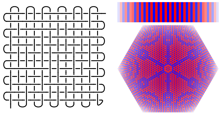
FIGURE 1.3. \Theta of a randomized weave knot, as computed by Self [BV3, WeaveKnots.nb]. Crossings were chosen to be positive or negative with equal probabilities.
