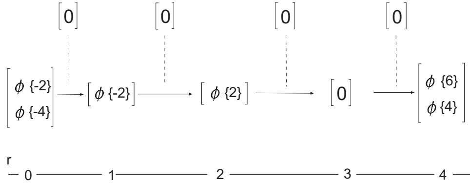
Figure 8. A closure of a coherently diagonal complex is a width-two complex.
