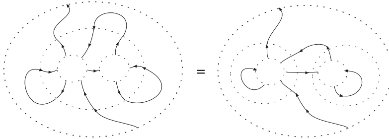
Figure 3. The closure of a binary operator can be considered as the binary composition of two unary operator closures
