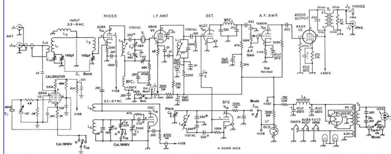
Circuit diagram of the 6X2 Super-heterodyne. Unless indicated otherwise, decimal capacitances are in \mu\text{f} , other capacitances in \mu\text{mfd} , resistors are \frac{1}{2} watt.
