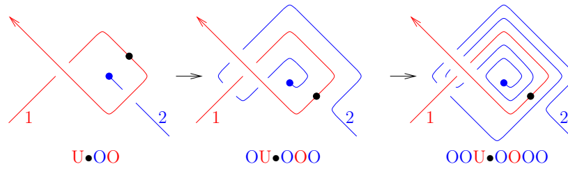
FIGURE 22. Attempting to fix a non-OU tangle diagram in the virtual [Kal] / Kauffman:VirtualKnotTheory tangloid [Tu] case.
