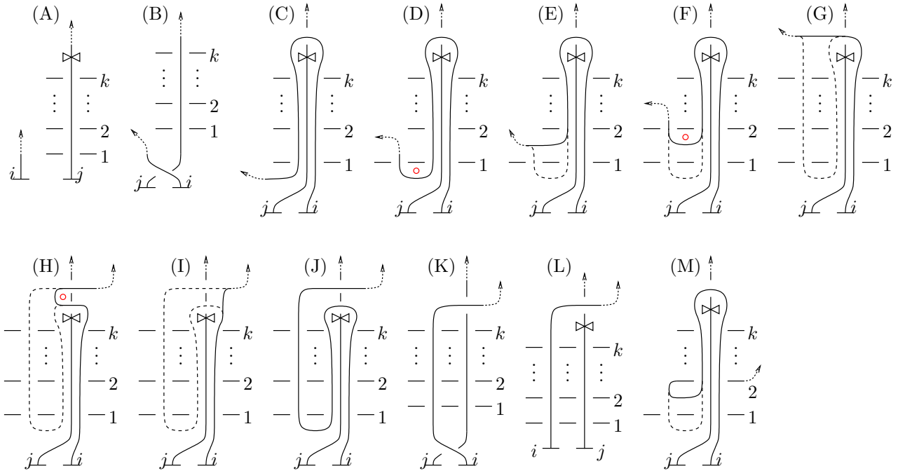
FIGURE 19. Proof of the “only if” side of Lemma 7.1 . lem:div
