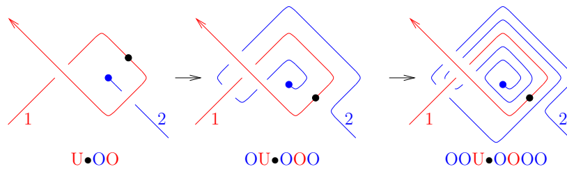
FIGURE 22. Attempting to fix a non-OU tangle diagram in the virtual tangloid [Tu] case. [Kauffman:VirtualKnotTheory]
