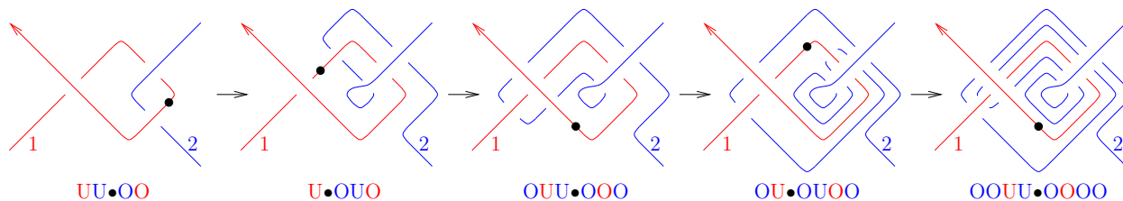
FIGURE 5. An attempt to fix a non-OU tangle diagram. In each step we use a single glide move to fix the first UO sequence encountered on strand 1 (we mark it with a \bullet ), but things get progressively more complicated. The O/U sequences below the diagrams are listed from the perspective of strand 1.
