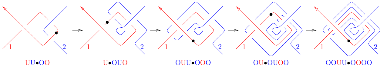
FIGURE 5. An attempt to fix a non-OU tangle diagram. In each step we use a single glide move to fix the first UO sequence encountered on strand 1 (we mark it with a \bullet ), but things get progressively more complicated. The O/U sequences below the diagrams are listed from the perspective of strand 1.
