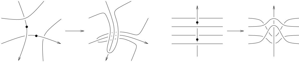
FIGURE 3. Two possibilities for “interacting” UO intervals (each marked with a • symbol).
