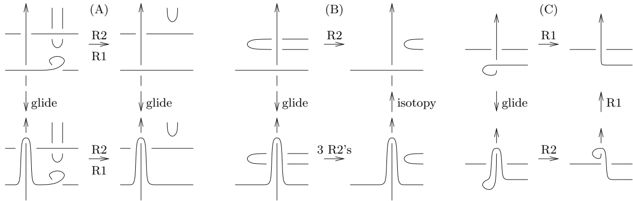
FIGURE 4. R1 and R2 moves “commute” with glides (A), or they make glides redundant (B), (C).
