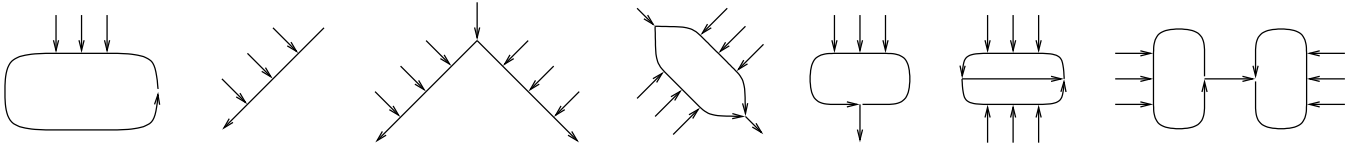
Figure 5. Primitives in \mathcal{A}_k^{vc} with at most one “co” vertex, ignoring some IHX -reducibles. To complete these pictures, all loose ends in these diagrams must be connected to the k skeleton lines \uparrow\uparrow \dots \uparrow in an arbitrary manner.
