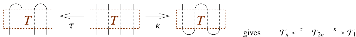
Figure 3. The definitions of \tau and \kappa .
