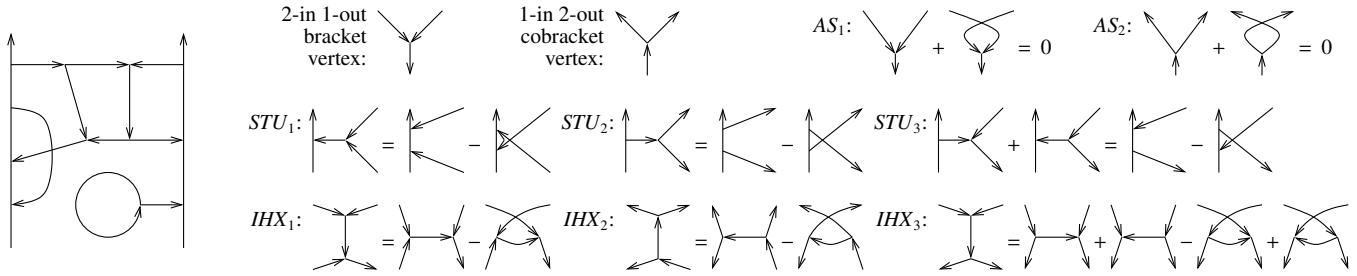
Figure 4. \mathcal{A}^{vc} in some detail: a typical diagram, then the two types of internal trivalent vertices, then the AS, STU, and IHX relations. \mathcal{A}^{vc} is \mathbb{Q}(\text{such diagrams}) / (AS, STU, IHX) .
