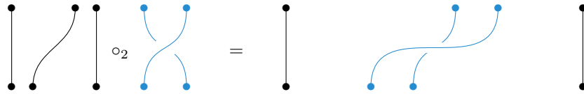
Figure 2.5.2: Partial composition operations in PaB . For two parenthesized braids P_1 and P_2 , P_1 \circ_i P_2 is obtained by shrinking P_2 down so that the strands in P_2 are closer together than any two strands in P_1 and then replacing the i th strand of P_1 with P_2 .
