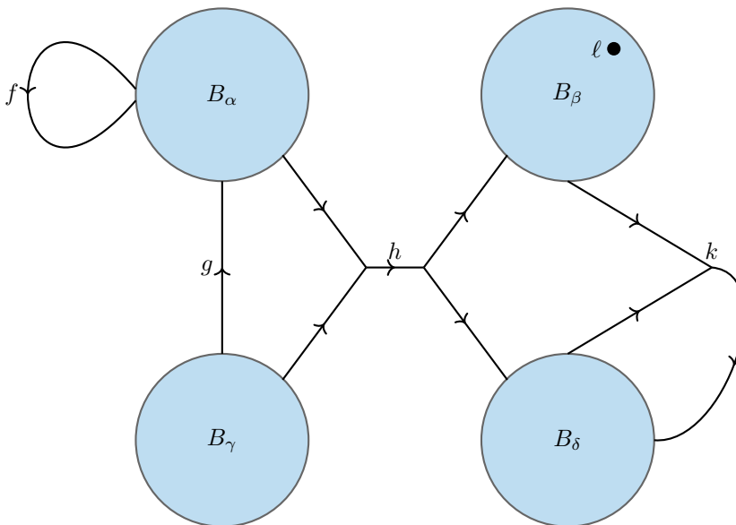
Figure 2.1.1: An example of an algebraic structure comprising four objects B_\alpha, B_\beta, B_\gamma, B_\delta , four operations f : B_\alpha \rightarrow B_\alpha, g : B_\gamma \rightarrow B_\alpha, h : B_\alpha \times B_\gamma \rightarrow B_\beta \times B_\delta and k : B_\beta \times B_\delta \rightarrow B_\delta between the various objects and a nullary operation \ell : \star \rightarrow B_\beta which is a choice of constant in B_\beta .
