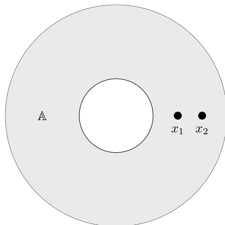
Figure 3.1.1: The basepoint for \text{Conf}_n(\mathbb{A}) is n evenly spaced points lying on the portion of the x -axis to the right of the core of the annulus as indicated for \text{Conf}_2(\mathbb{A}) .
