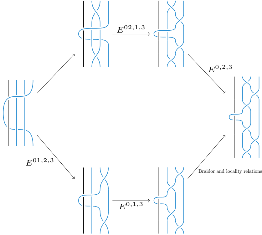
Figure 3.5.1: The derivation of an equation satisfied by the error E in the mixed relation in degree n + 1 . Start at the left-most chord diagram in the figure, then follow the two paths to the right-most diagram. Each time the slide relation must be applied, to get from one diagram to the next, the corresponding error term accrued is written above the error. Summing over the error terms along each path and setting the result to be equal since we end on the same diagram yields the equation E^{01,2,3} - E^{0,2,3} - E^{02,1,3} + E^{0,1,3} = 0
