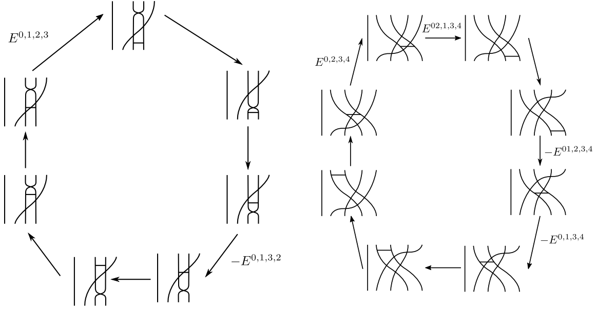
Figure 3.6.1: The derivation of the syzygies S1 and S2. Start at any chord diagram in the figure, then follow the entire loop indicated by the arrows back to the start. Each time the slide relation must be applied, to get from one diagram to the next, the corresponding error term accrued is written above the arrow. Summing over all these error terms and setting the result equal to zero in the left diagram yields the equation E^{0,1,2,3} = E^{0,1,3,2} while doing this for the right diagram yields E^{0,2,3,4} + E^{02,1,3,4} = E^{0,1,3,4} + E^{01,2,3,4} .
