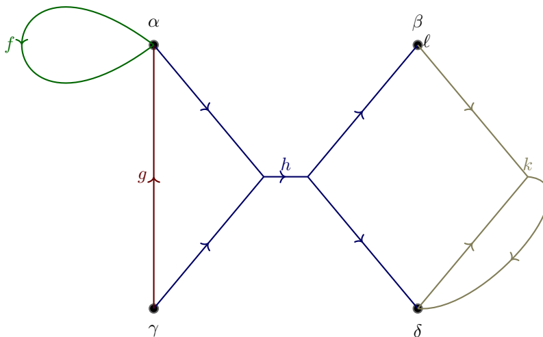
Figure 2.1.2: The multigraph underlying the algebraic structure in Figure 2.1.1. Some of the vertices are labelled in Greek letters by the types of the algebraic structure, although some vertices are unlabelled. The oriented edges of the graph come from the operations in the algebraic structure and each edge is labelled by the operation it comes from, indicated via colour coding. Constants are indicated by adding an extra label in the Latin alphabet to a vertex.
