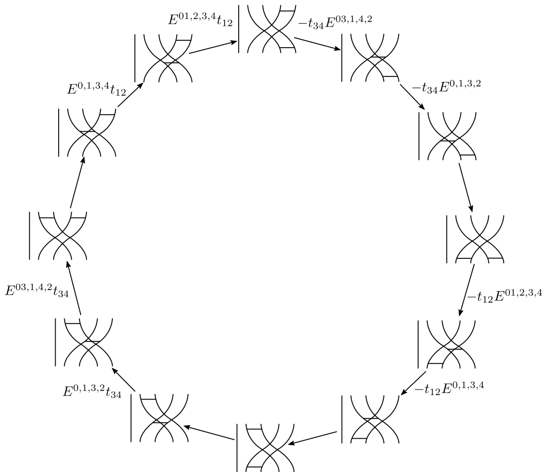
Figure 3.6.2: The derivation of the syzygy S3. Start at any chord diagram in the figure, then follow the entire loop indicated by the arrows back to the start. Each time the slide relation must be applied, to get from one diagram to the next, the corresponding error term accrued is written above the error. Summing over all these error terms and setting the result equal to zero yields the equation [E^{0,1,3,4} + E^{01,2,3,4}, t_{12}] + [E^{0,1,3,2} + E^{03,1,4,2}, t_{34}] = 0 .
