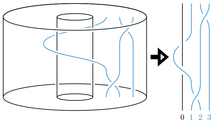
Figure 3.1.2: An annular braid with 3 strands and underlying permutation (132) as well as its representation as a usual 4 strand braid with distinguished 0th strand remaining fixed.
