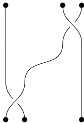
Figure 2.5.1: A parenthesized braid. This is a morphism in the groupoid \mathbf{PaB}(3) from the object (\bullet\bullet)\bullet to the object \bullet(\bullet\bullet) .
