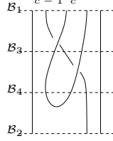
FIGURE 42. To define \mathcal{U}^c , tensor \mathcal{U}^{c-1} with \mathcal{P}^c and \mathcal{P}^{c-1} , as shown.
