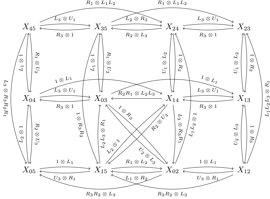
FIGURE 34. \mathcal{B}_3 \mathcal{P}_{\mathcal{B}_2}^2 \boxtimes^{\mathcal{B}_2, \mathcal{B}'_1} \mathcal{P}_1 when \{1, 2, 3\} \subset \mathcal{S}
