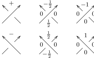
FIGURE 2. Sign conventions for crossings, and local Alexander and Maslov contributions. The first column illustrates the chirality of a crossing; the second the Alexander contribution of each quadrant; the third the Maslov contribution.
