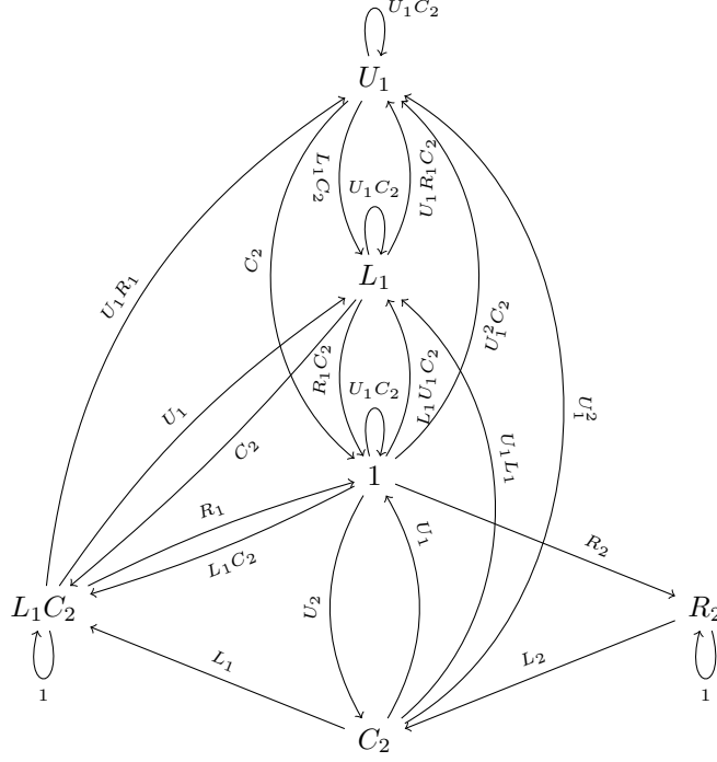
FIGURE 40. Operation graph for a minimum when 2 \in \mathcal{S}_1 .
