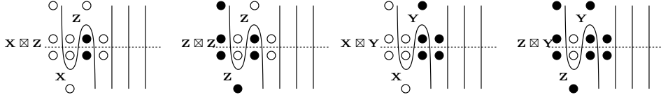
FIGURE 47. Generator types for \mathcal{B}_1 \cup_{\mathcal{B}_2}^1 \boxtimes^{\mathcal{B}_2} \Omega_{\mathcal{B}_1}^2 .
