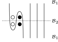
FIGURE 46. Generators of \mathcal{B}_1 \cup_{\mathcal{B}_2}^1 \boxtimes^{\mathcal{B}_2} \Omega_{\mathcal{B}_1}^2 . Generators correspond to the idempotents in the incoming algebra \mathcal{B}_1 ; the constraints on the intermediate generators are as shown.
