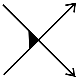
Figure 4 - A Black Hole
