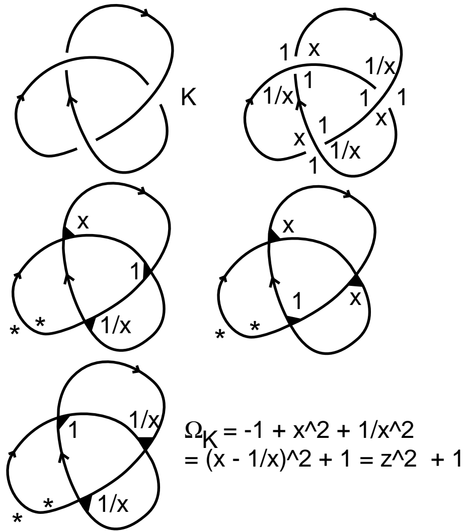
Figure 12 - Conway Calculation.
