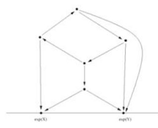
FIGURE 3. Wheel type graph with symbol \Gamma(x, y) = \text{tr}(y^2[x, y]x) .
