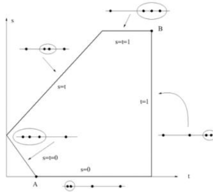
FIGURE 11. The compactification space of 4 positions on a line
