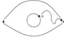
FIGURE 8. A simple path from Duflo-Kontsevich star product to standard product
