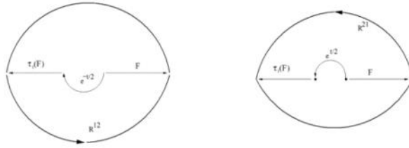
FIGURE 9. The R matrix
