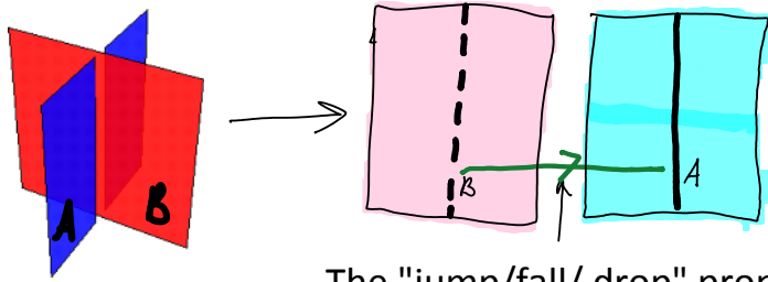
The "jump/fall/ drop" propagator
