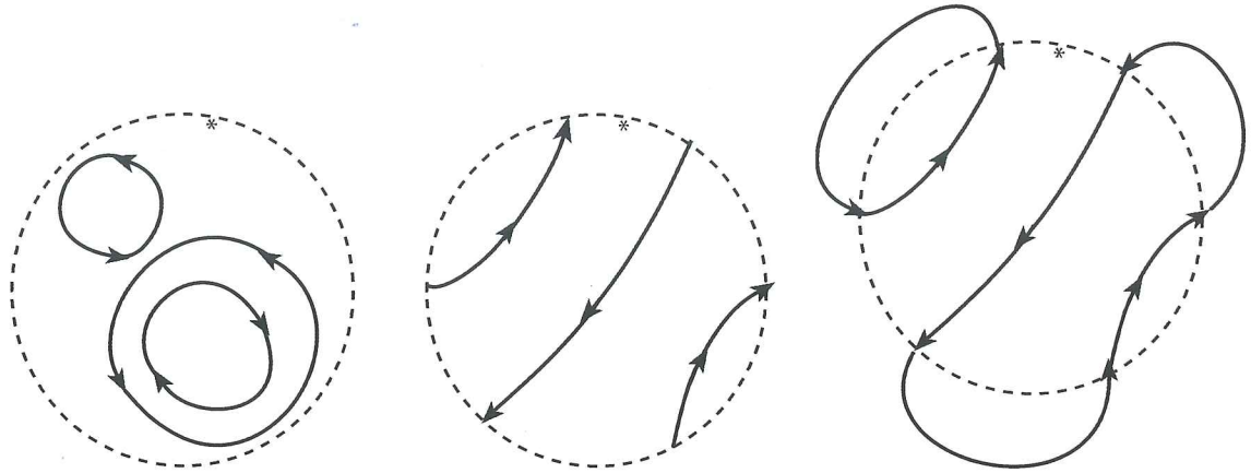
(A) Smoothing with rotation number 1 (B) Smoothing with rotation number 2 (C) The standard closure of the smoothing in B
