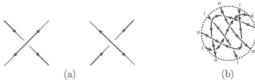
Figure 4. (a) Gravity information in a neighbourhood of a crossing. (b) Gravity information in the tangle. We use: o for out-boundary points and i for in-boundary points.
