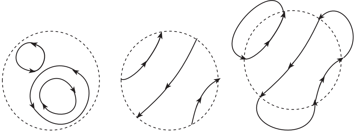
(A) Smoothing with rotation number 1 (B) Smoothing with rotation number 2 (C) A positive closure of the smoothing in b
